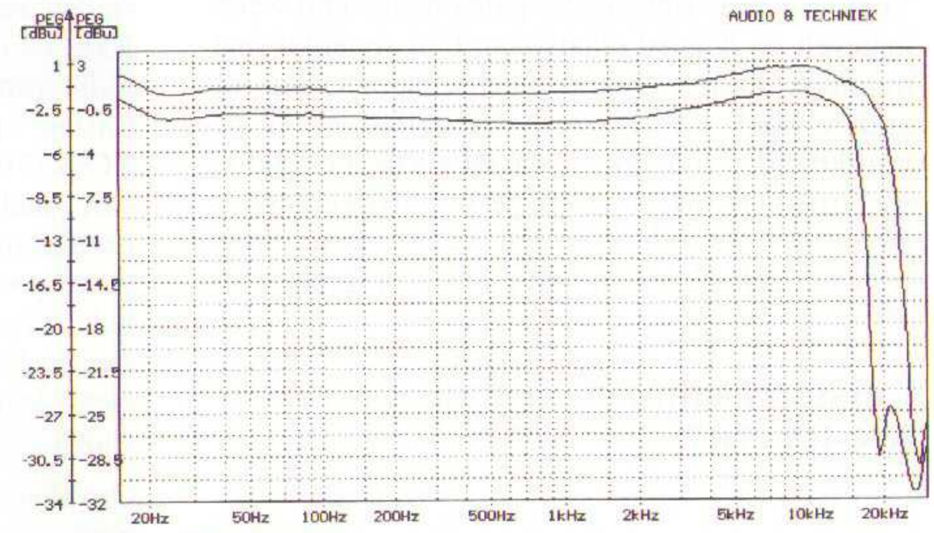
Sony TC-K670
